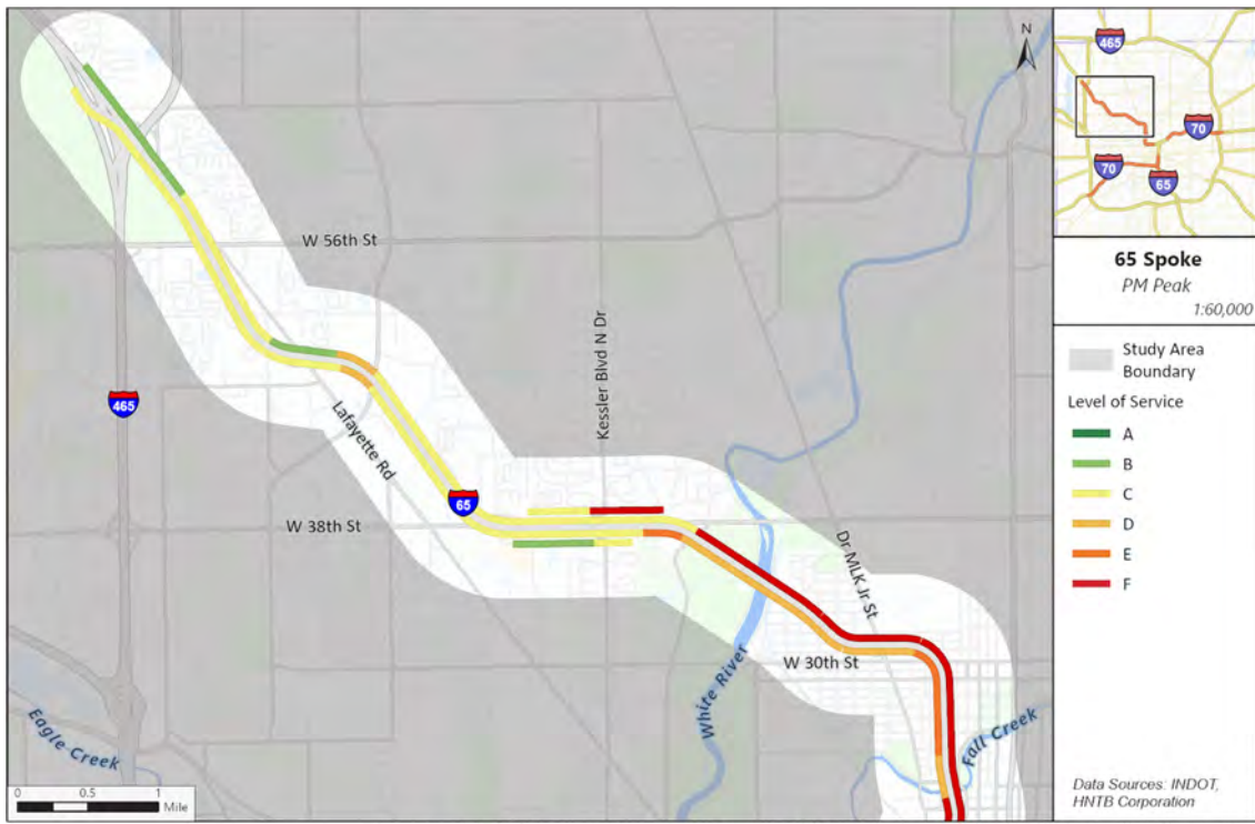
Figure 26: 65 Spoke Future (2050) Interstate Operations (PM Peak Hour)
