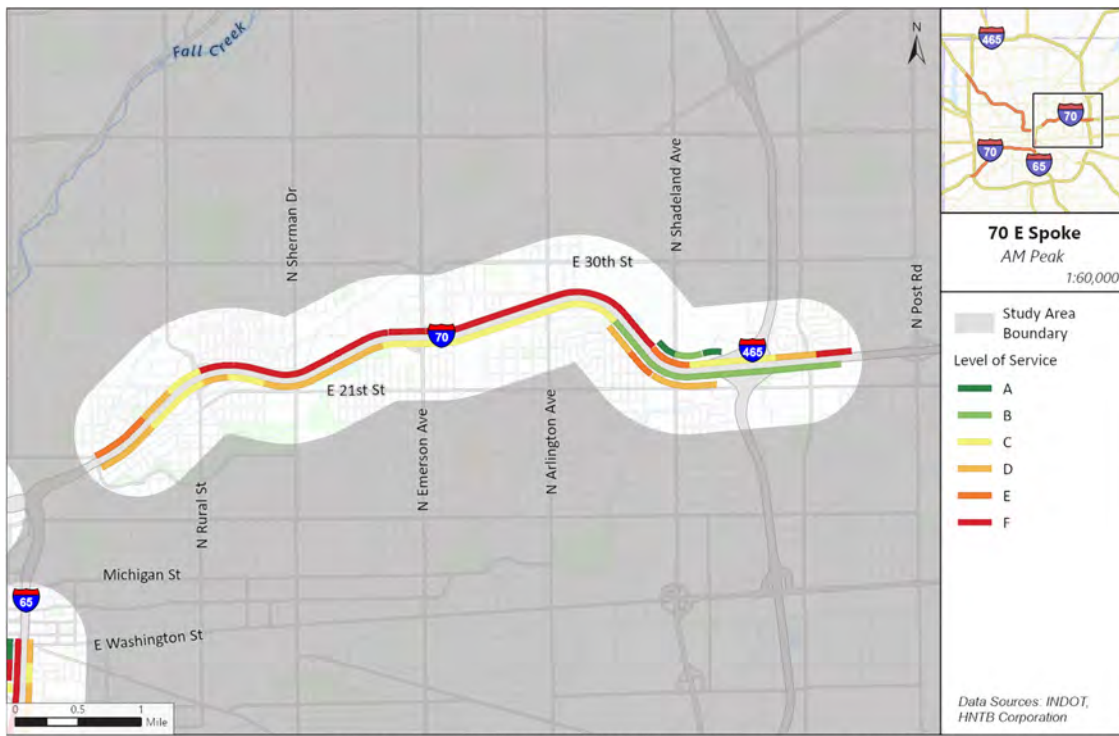
Figure 36: 70 E Spoke Future (2050) Interstate Operations (AM Peak Hour)
