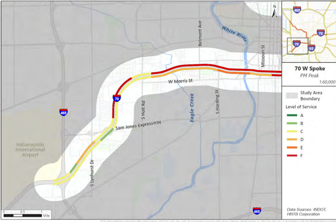
Figure 34: 70 W Spoke Future (2050) Interstate Operations (PM Peak Hour)
